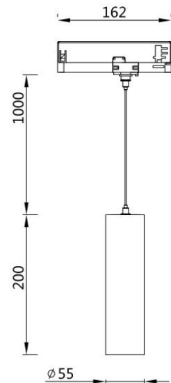
Honeycomb Oval diffuser Diffuser Anti-glare ring
